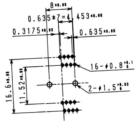
P.C.B. PATTERN (TOP VIEW)
