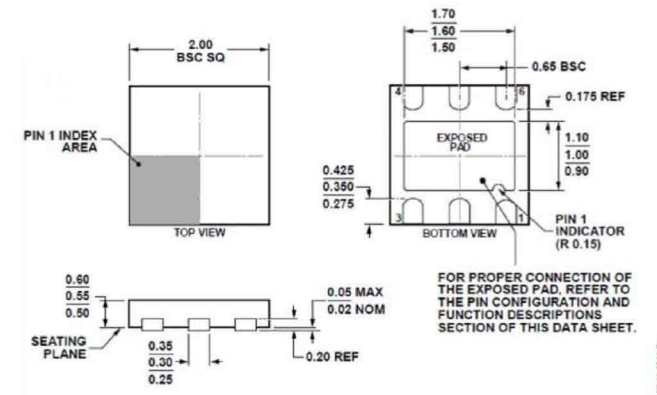
Figure 55. 6-Lead Lead Frame Chip Scale Package [LFCSP_UD] 2.00 mm x 2.00 mm Body, Ultra Thin, Dual Lead (CP-6-3) Dimensions shown in millimeters
