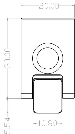
SOCKET TOP VIEW
