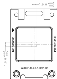
LIMIT BOX TOP VIEW
