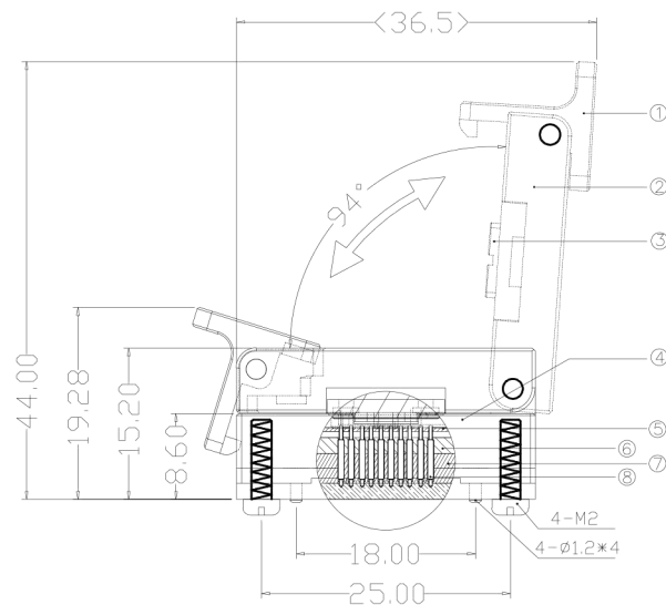
SOCKET RIGHT VIEW
