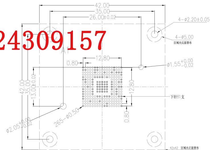
PCB PATTERN (Top View)
