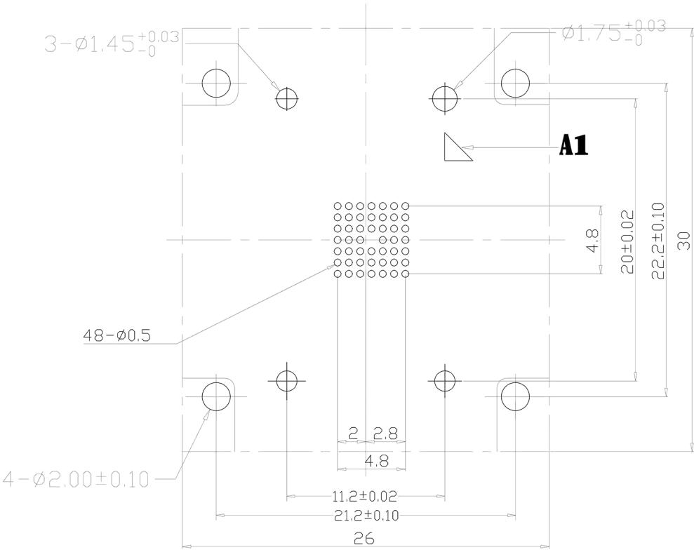
PCB Pattern(TOP View)
