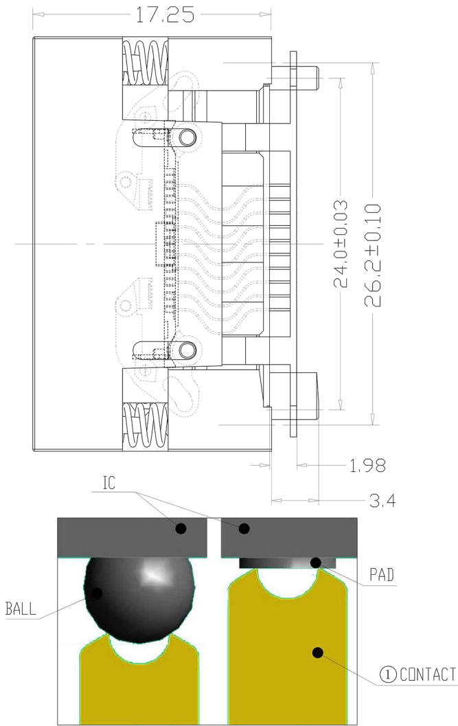
CONTACT TIP DETAIL
