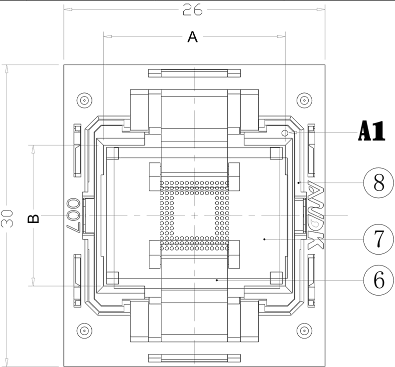
IC Loading Direction (Center In)
