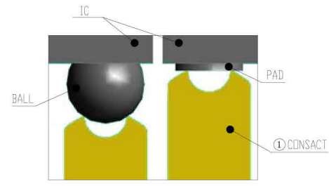
CONSAC TIP DETAIL
