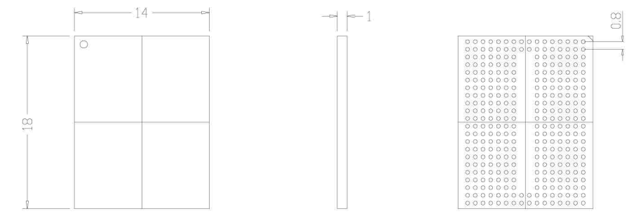
TOP VIEW SIDE VIEW BOTTOM VIEW
