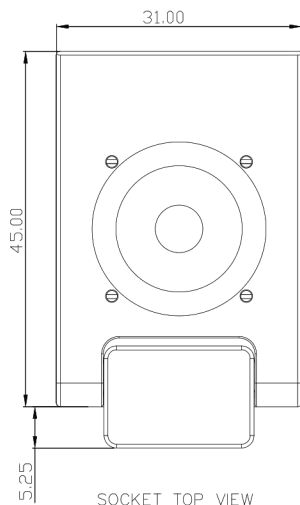
SOCKET TOP VIEW
