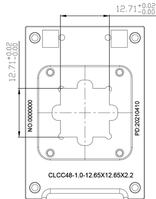
LIMIT BOX TOP VIEW
