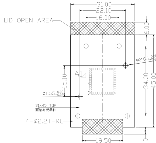
PCB PATTERN (Top View)
