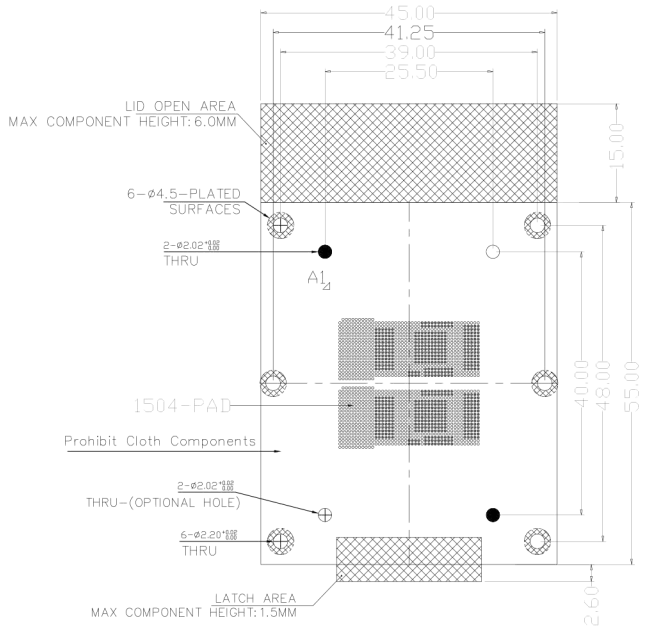
PCB PATTERN (Top View)
