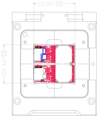
LIMIT BOX TOP VIEW
